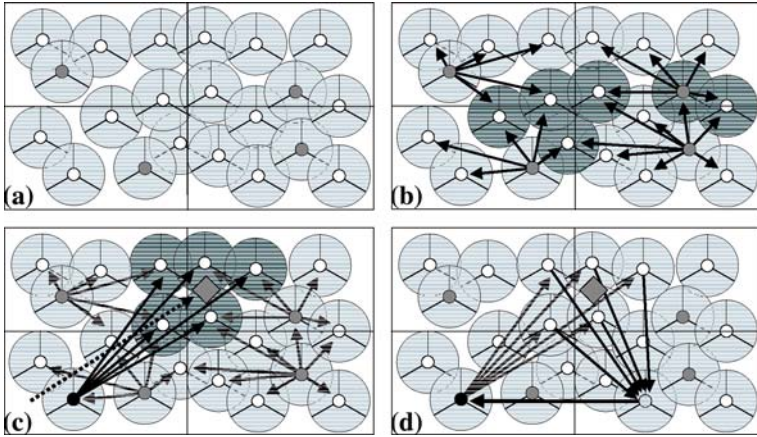
Figure 2. High-level distributed sensor allocation architecture. (a) shows the initial sensor layout, decomposition and allocation of sector managers. (b) shows the dissemination of scanning tasks. The new track manager in (c) can be seen coordinating with sensors to track a target, while the resulting data is propagated in (d) for processing.
