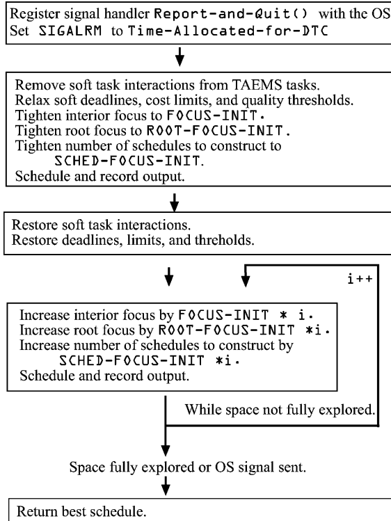
Figure 8. Real-time control for DTC.
