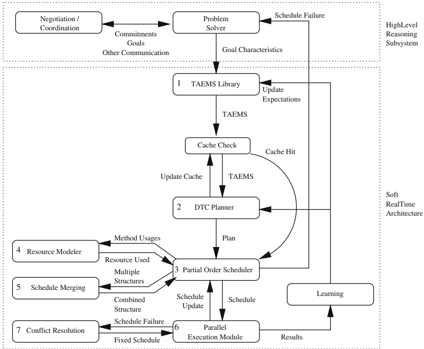
Figure 1. High-level agent control architecture.
