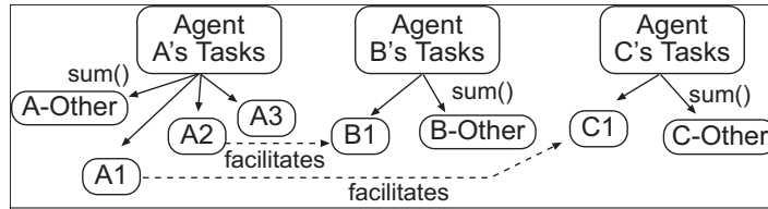
Figure 8 - Agent A 's Revised View
