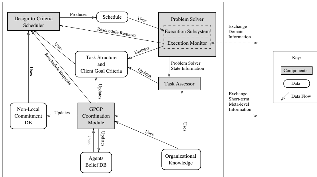
Figure 15: A Typical Agent Architecture
