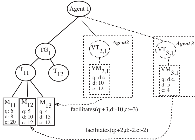
Figure 17: Example of agent reasoning about how best to contract for needed information from another agent
